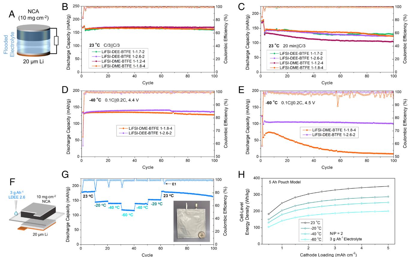
Fig. 6. Cycling behavior of Li metal full cells under reduced temperature of elevated charging rate. (A) Schematic of 20 μm Li || 10 mg cm -2 NCA coin-type full cells applied in (B–E). Cycling performance of cells at (B) 23 °C, C/3 charge || C/3 discharge and 4.3 V cutoff, (C) 23 °C, 20 min charge || C/3 discharge and 4.3 V cutoff, (D) -40 °C, C/10 charge || C/5 discharge and 4.4 V cutoff, (E) -60 °C, C/10 charge || C/5 discharge and 4.5 V cutoff. Cells in (D and E) are subjected to a single charge to 4.3 V at room-temperature before transferring to low-temperature. (F) Schematic and photo of single-layer 20 μm Li || 10 mg cm -2 NCA pouch-type full cells with 3 g Ah -1 LDEE 2.6 electrolyte. (G) Variable-temperature cycling of pouch-cell with 23 °C cycling at C/5 || C/3 and 4.3 V cutoff, -20 °C cycling at C/10 || C/5 and 4.3 V cutoff, -40 °C cycling at C/10 || C/5 and 4.4 V cutoff, and -60 °C cycling at C/20 || C/10 and 4.5 V cutoff. All cells use CC-CV charging with C/20 cutoff except for C, where the charge period is capped at 20 min, and G, where the low-temperature CV charge is capped at C/50. E1 refers to a cyler event in which the computer operating the battery cyler crashed and was not operating for ~3 d. (H) Cell-level energy density projections as a function of cathode loading and operating temperature (Materials and Methods).
