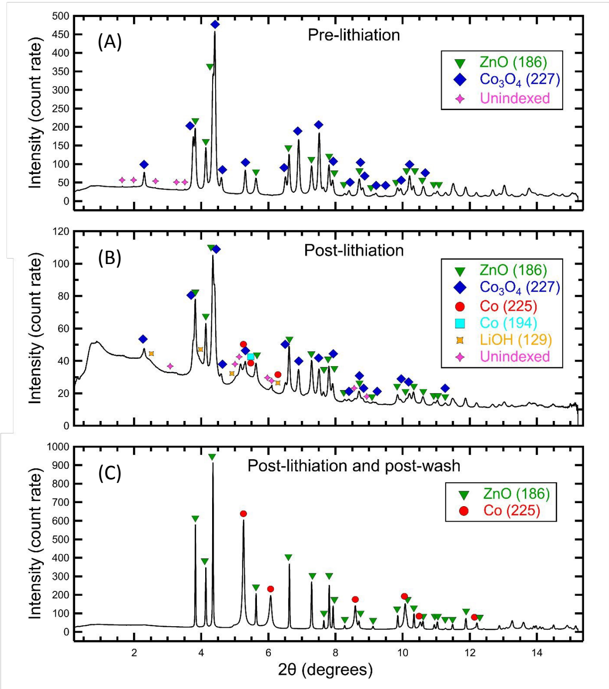
Figure 2. Phase identification results obtained from synchrotron XRD patterns for (a) the pre-lithiation precursor mixture of ZnO and \text{Co}_3\text{O}_4 , (b) the post-lithiation intermediate nanocomposite with a Li-containing phase, and (c) the post-lithiation and post-wash final NPo ZOC product.
