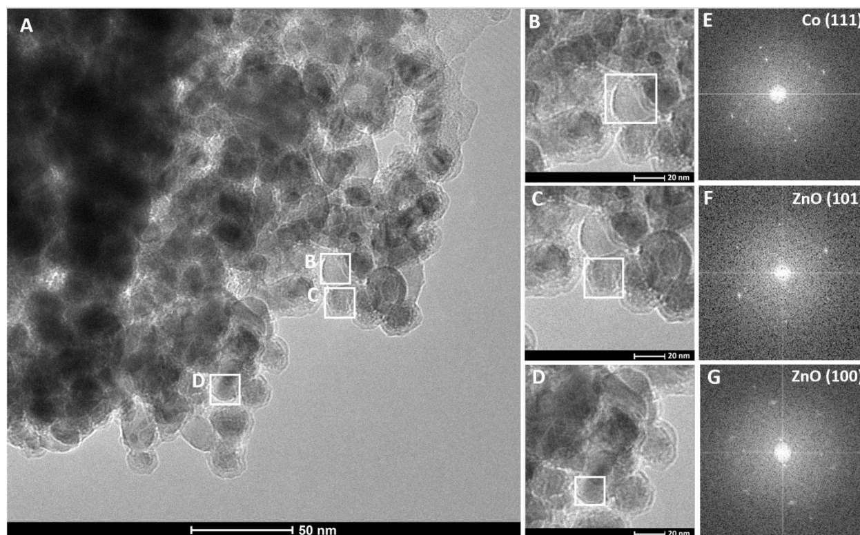
Figure 5. TEM images of post-lithiation and post-wash nanoporous ZnO-supported Co (A). NPo ZOC has primary particles on the order of 20nm, as was suggested by size-strain analysis of XRD data. The zoomed in regions of fcc Co and wurtzite ZnO (B, C, D) show selected area electron diffraction patterns (E, F, G) that confirm the structure of the ZnO and Co phases, as well as their close proximity demonstrating that they are very well intermixed.
